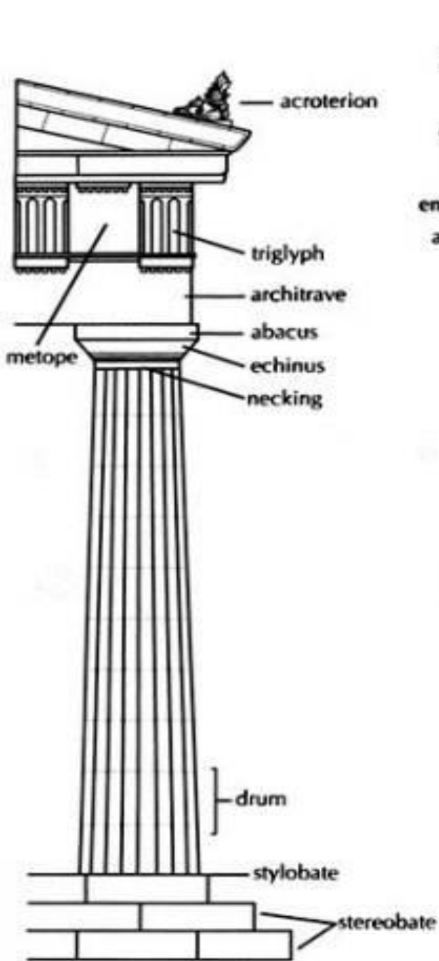
Doric order
